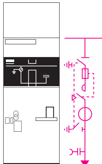
Fig. 27: Contactor-fusibles (750 mm).
